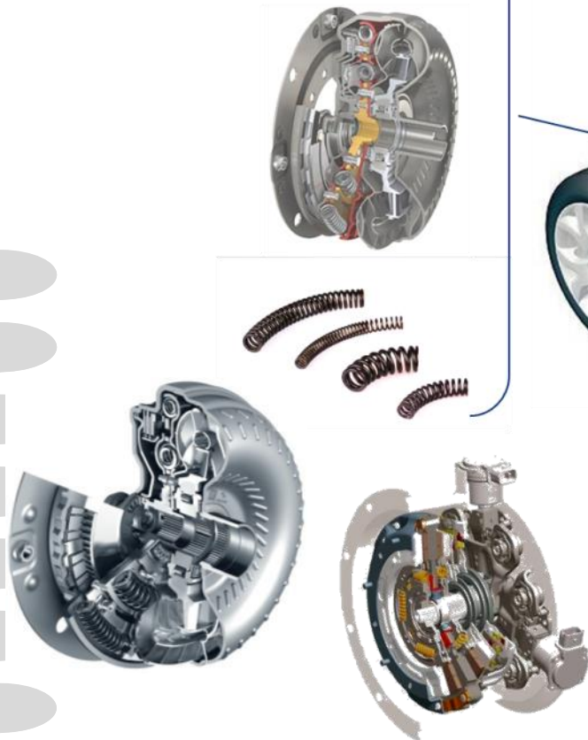
Torque Converter
